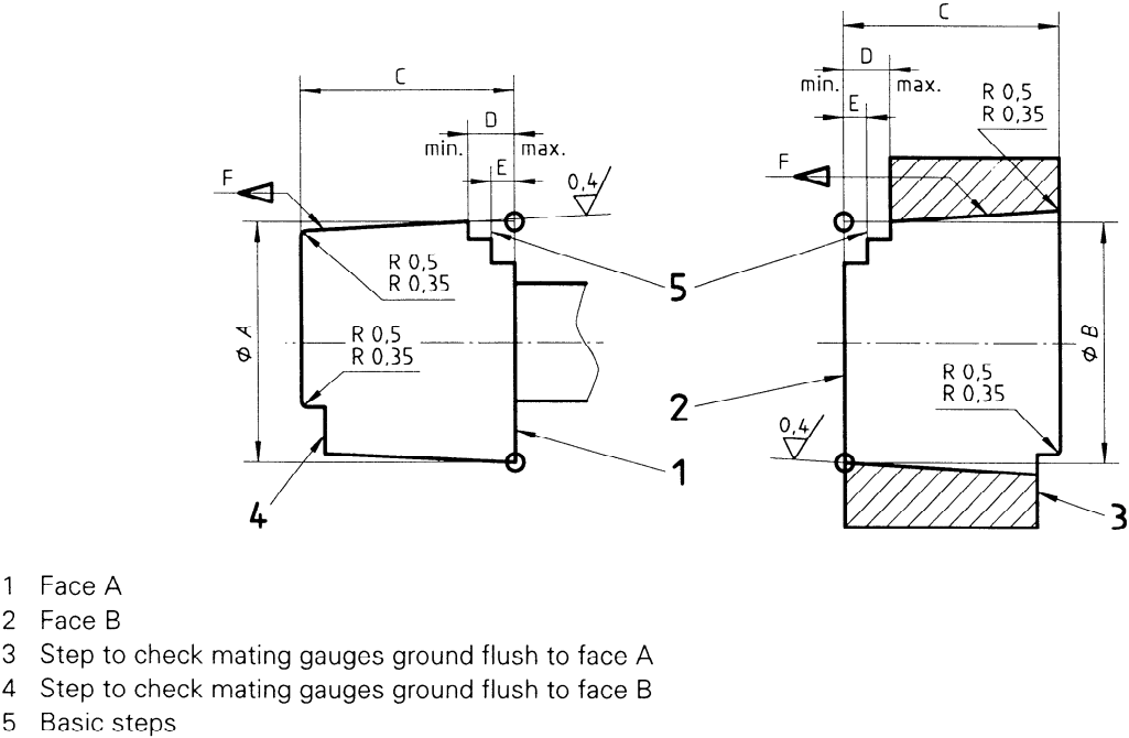
Figure E.1 — Plug and ring test gauges for conical connectors made of metal
